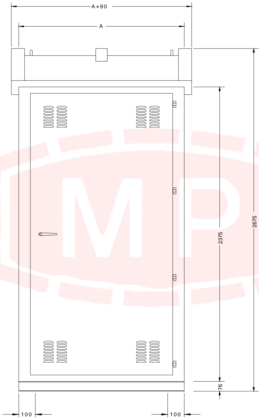
VISTA FRONTAL
